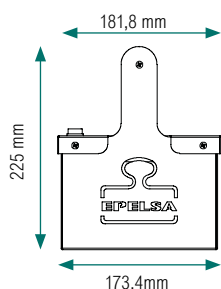
Battery holder Front view
